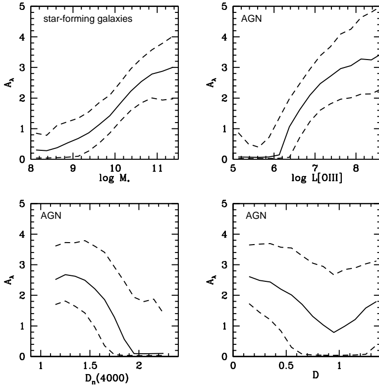
Figure 21: Top Left: The attenuation at [\text{OIII}]\lambda 5007 in magnitudes is plotted as a function of stellar mass for normal star-forming galaxies. Top Right: The attenuation is plotted as a function of [\text{OIII}] luminosity for AGN. Bottom: Attenuation in AGN hosts is plotted as a function of D_n(4000) (left) and distance parameter D (right). The solid line shows the median value of the attenuation, while the dashed lines show the 16-84 percentiles of the 1/V_{max} weighted distribution.
